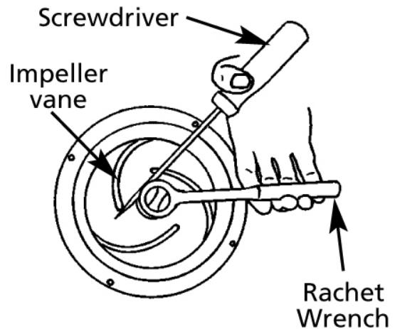
Figure 1 - Impeller Removal
