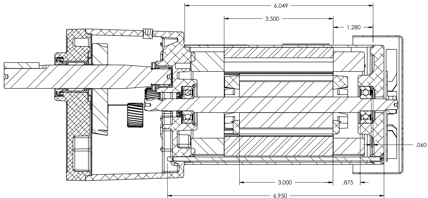
SECTION B-B
