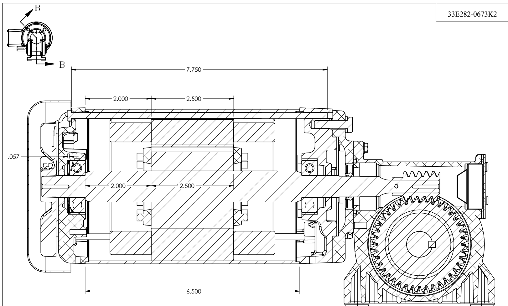
SECTION B-B
