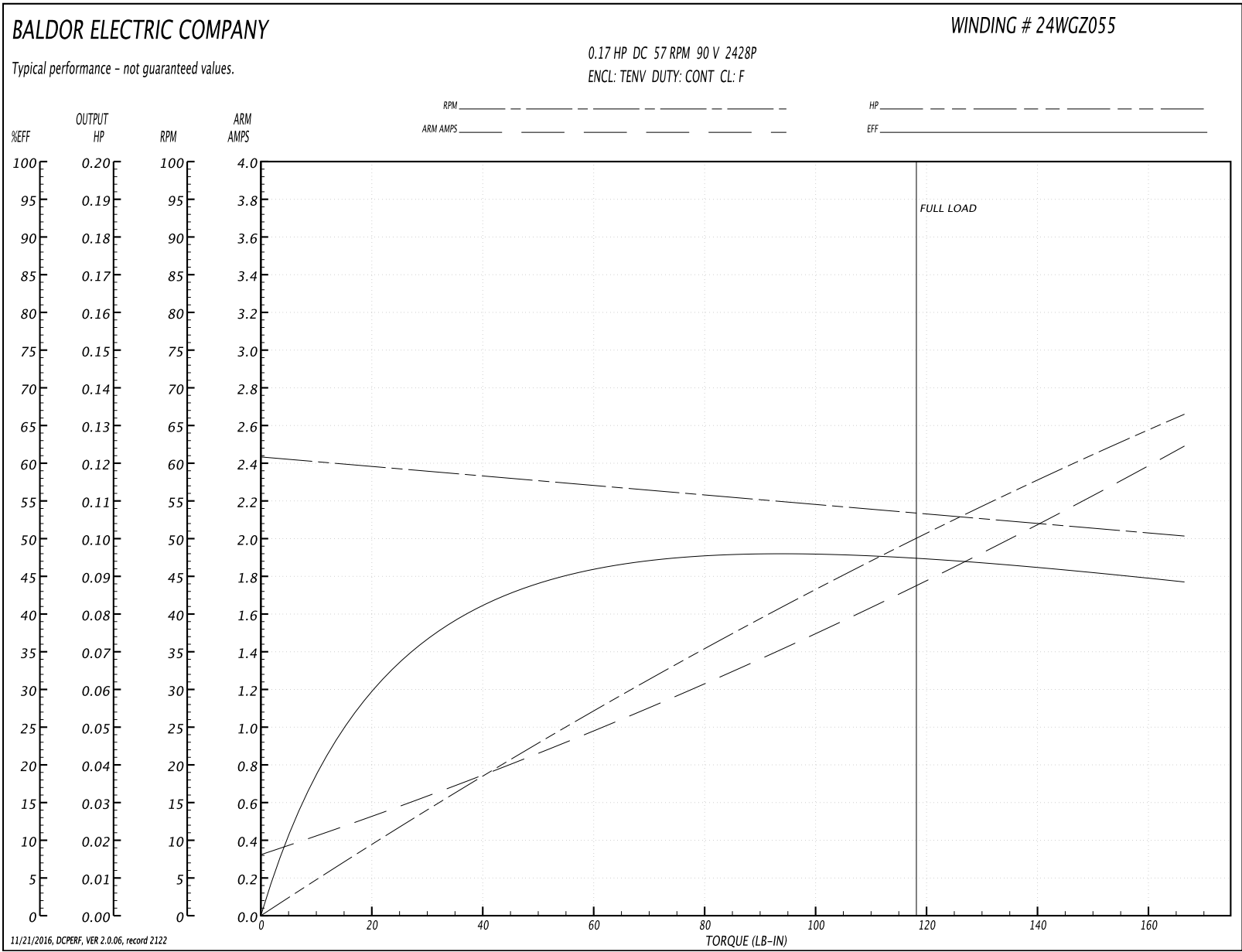
Performance Graph at 90.0 Arm V, 0.17HP Typical performance - Not guaranteed values
