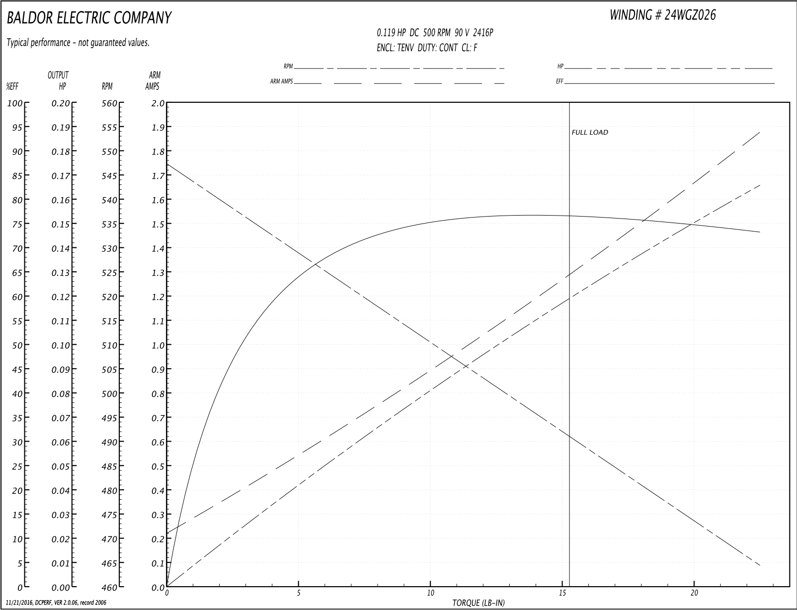
Performance Graph at 90.0 Arm V, 0.119HP Typical performance - Not guaranteed values
