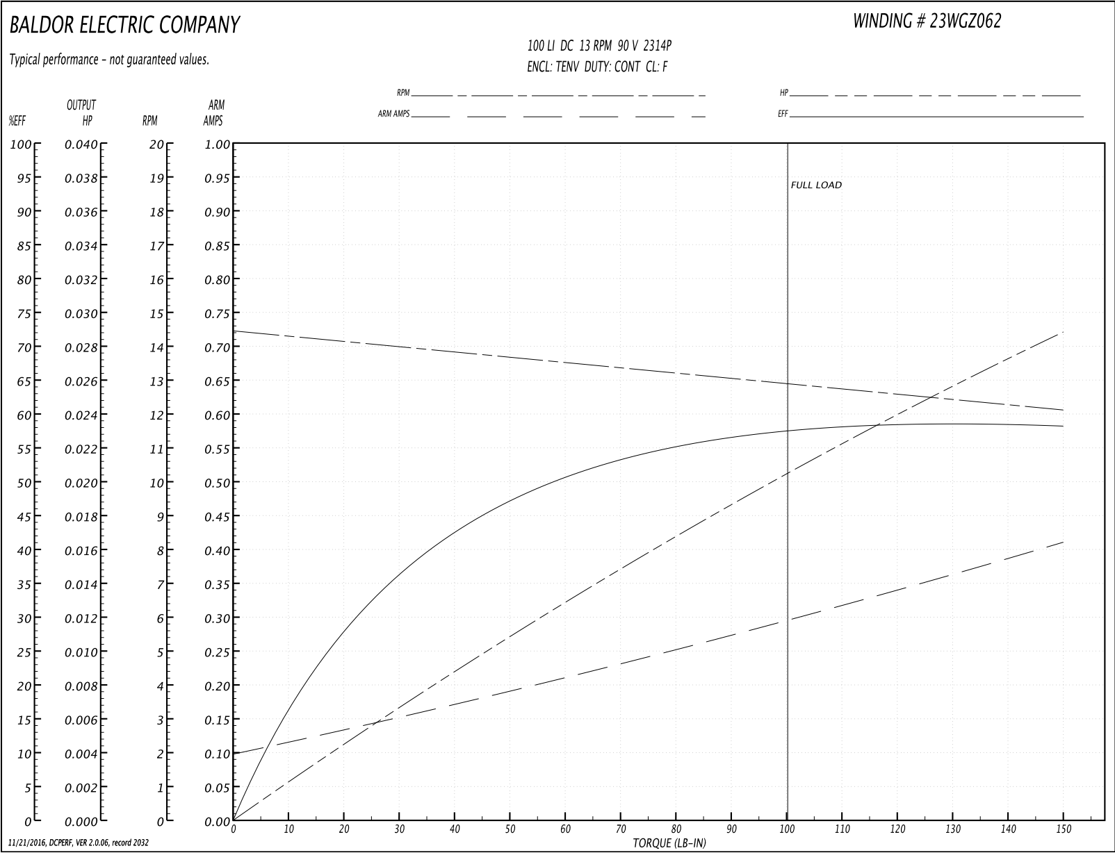
Performance Graph at 90.0 Arm V, 100.0LI Typical performance - Not guaranteed values
