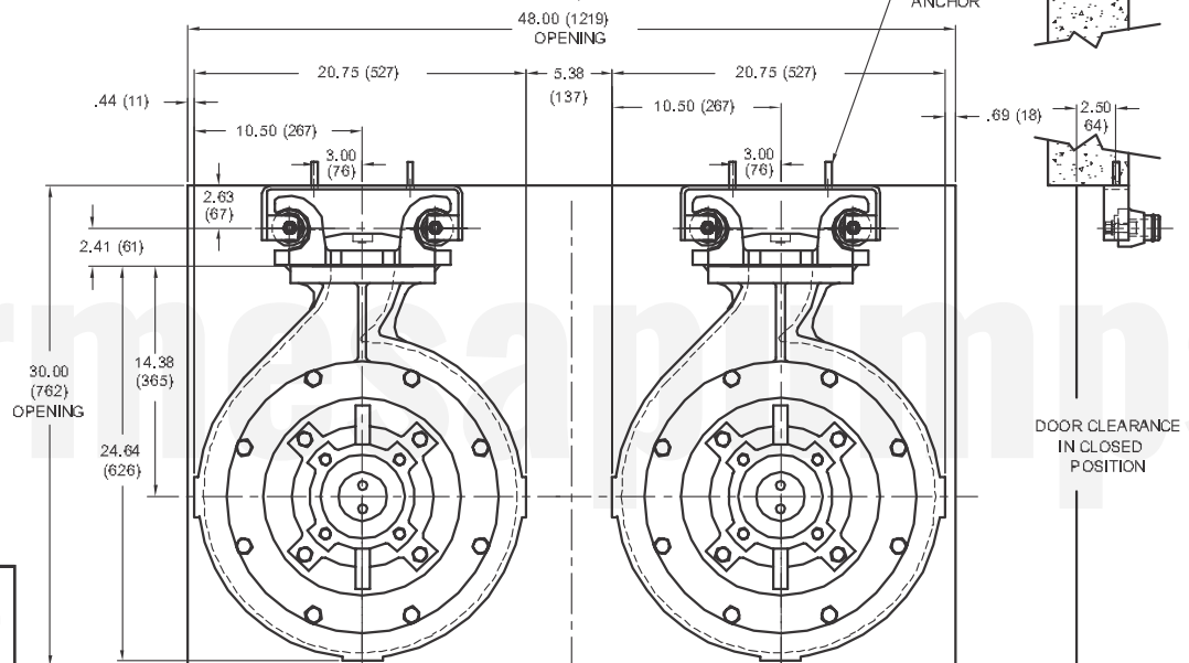
Figure 4 Duplex Installation (Standard)
