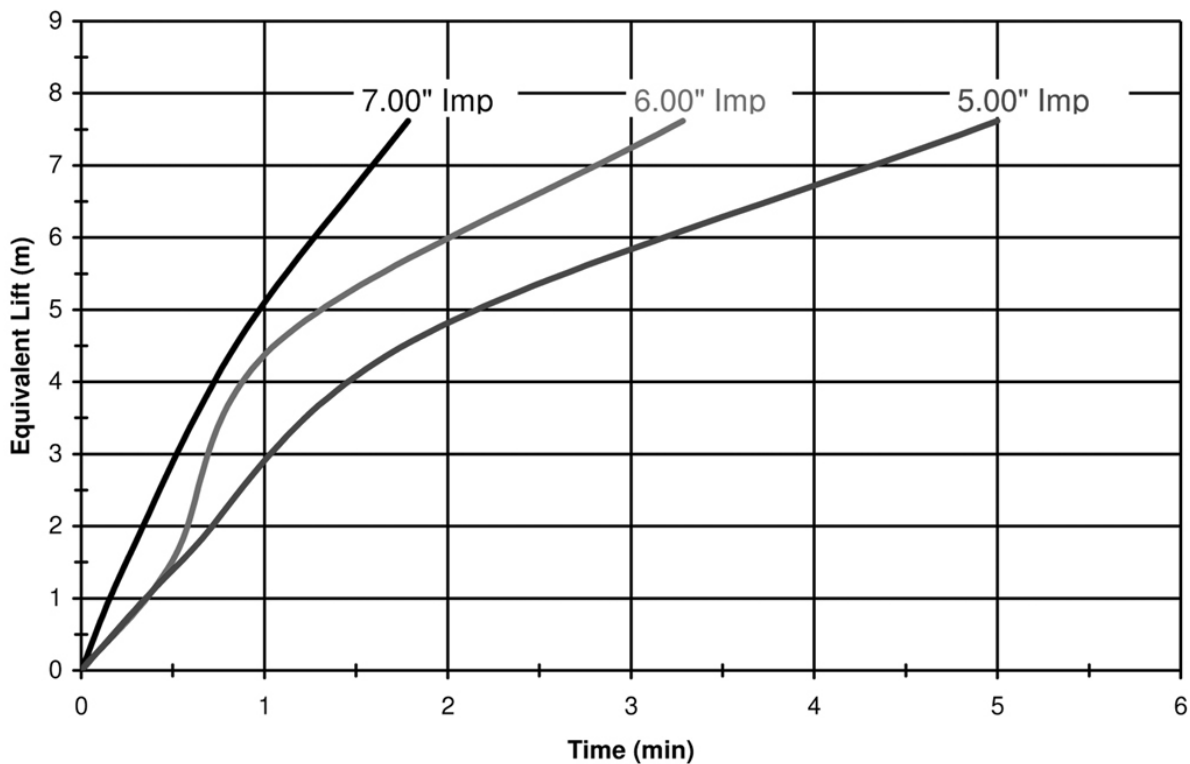
SP22 Prime Time- 2900 RPM 2" Suction Pipe
