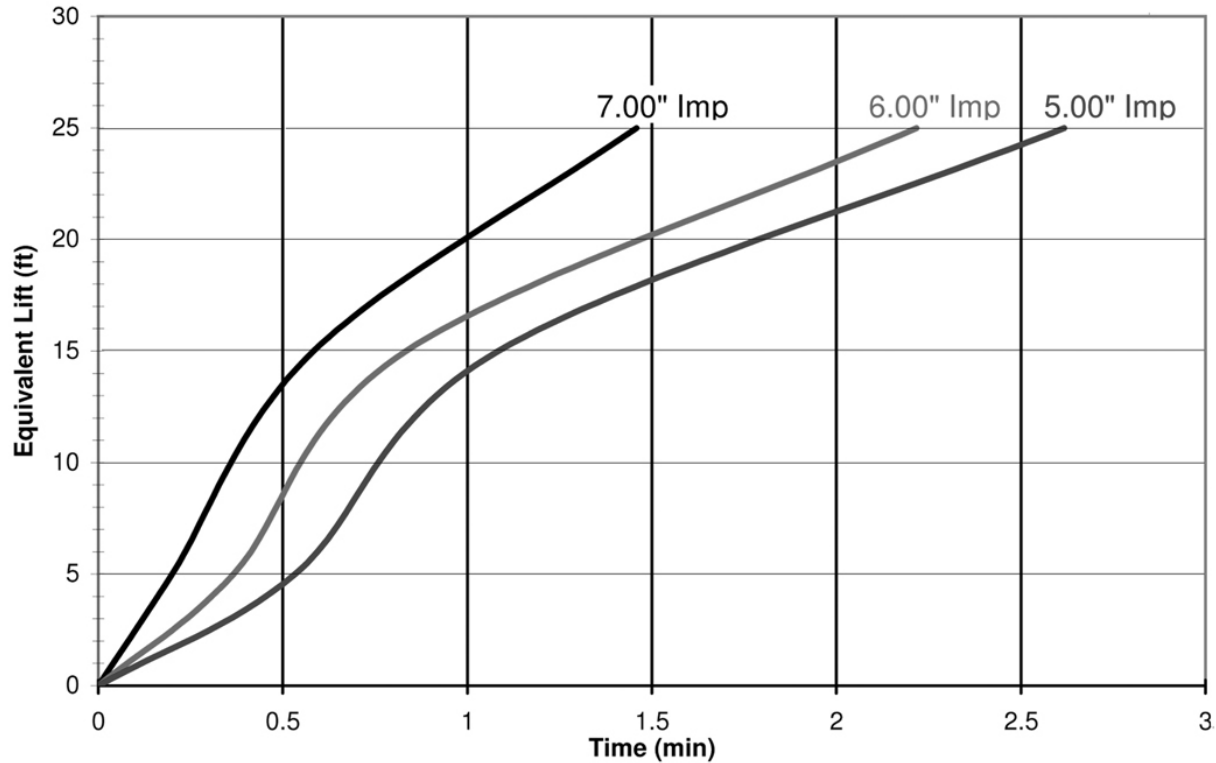
SP22 Prime Time- 2900 RPM 2" Suction Pipe
