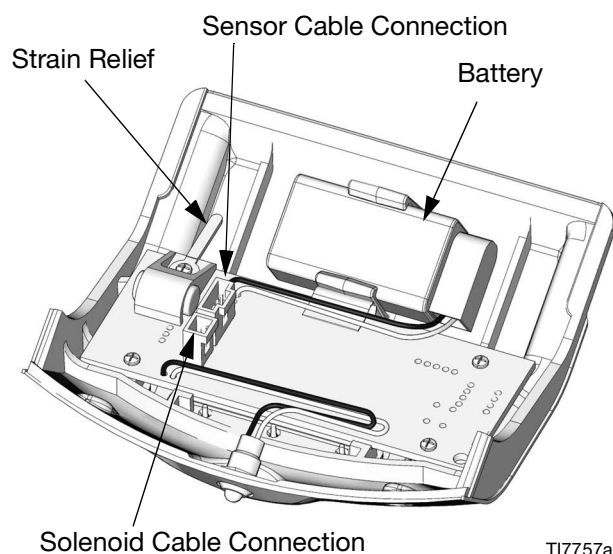
FIG. 1. Battery Location and Module Cable Connections
