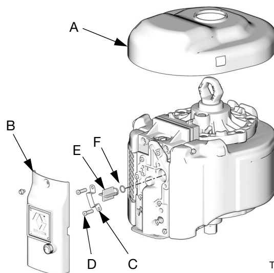
FIG. 2. Disassembly
