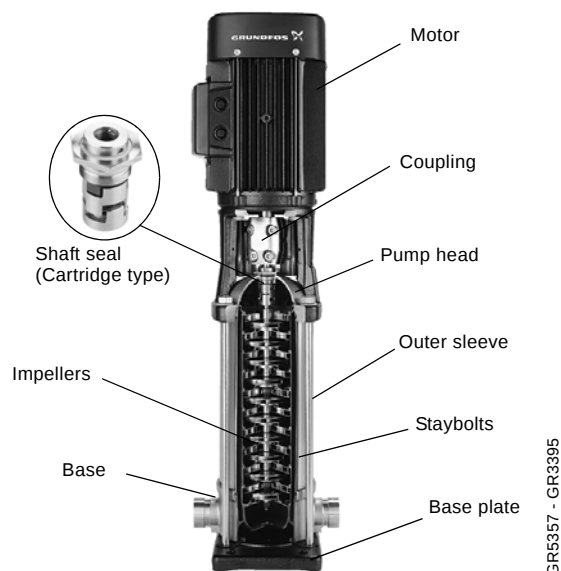
Fig. 3 CR pump
