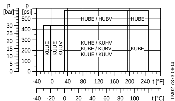
Fig. 15 Operating range of standard shaft seals for CR 32 - CR 150 (3.0-60 Hp)
