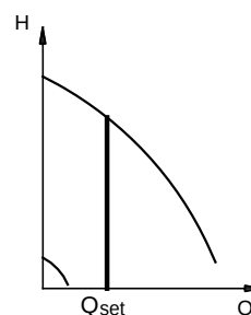
Fig. 12 Constant flow mode
