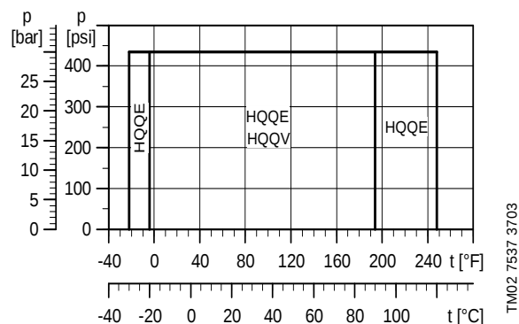
Fig. 14 Operating range of standard shaft seals for CR 1s - CR 20
