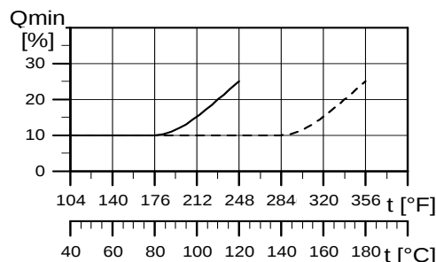
Fig. 28 Minimum flow rate
