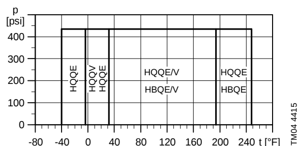
Fig. 16 Operating range of standard shaft seals for CR 120 - CR 150 (75-100 Hp)
