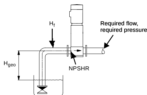
Fig. 18 Sizing data
