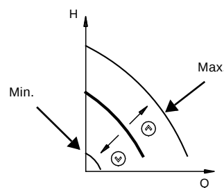
Fig. 13 Constant curve mode
