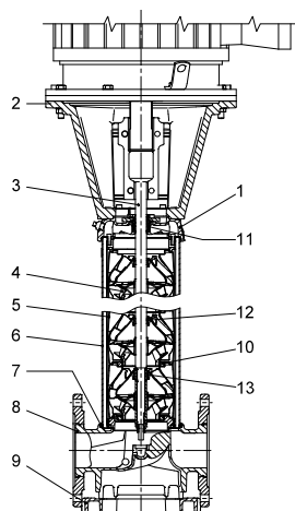
Sectional drawing
