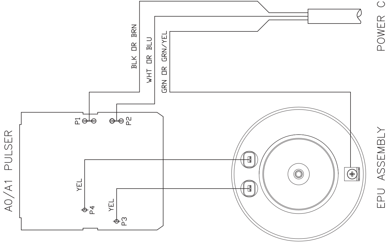
Series A0/A1 Wiring Diagram
