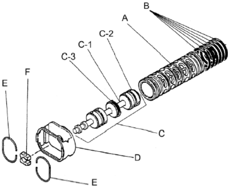
803115 C-Spool Valve Assembly (5-13-12)
